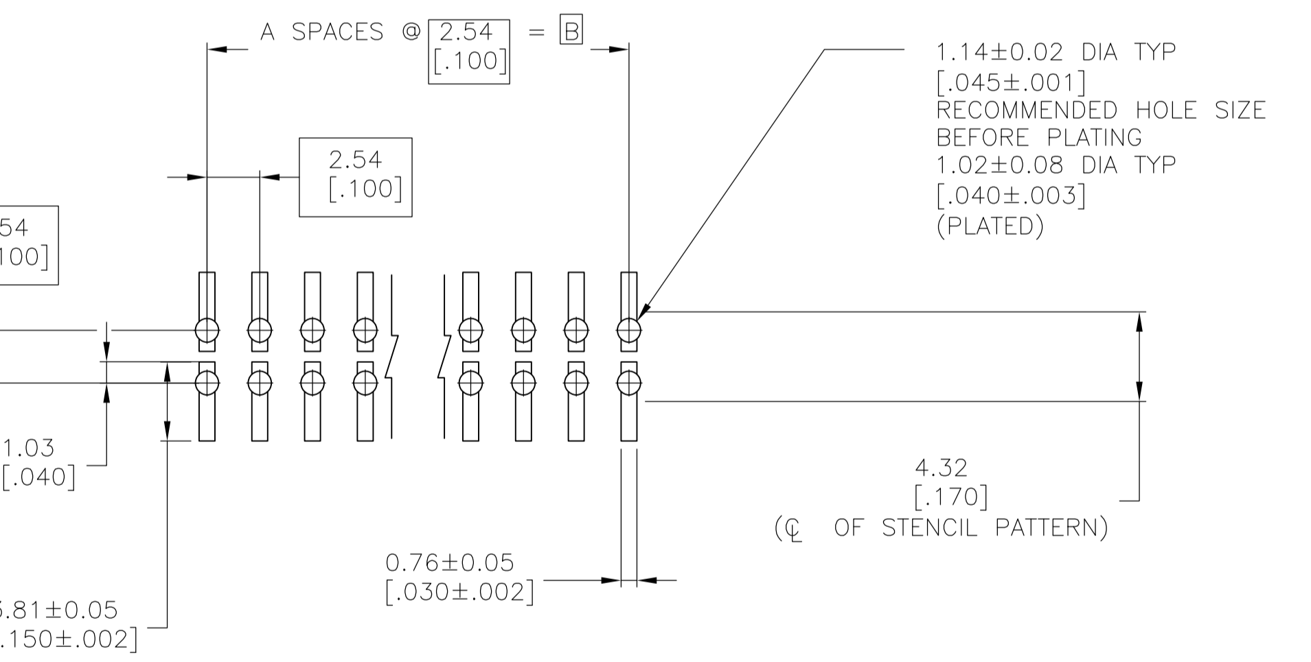
RECOMMENDED PC BOARD MOUNTING DIMENSIONS FOR .063[.160] THICK PC BOARD AND .012[.305] STENCIL THICK
