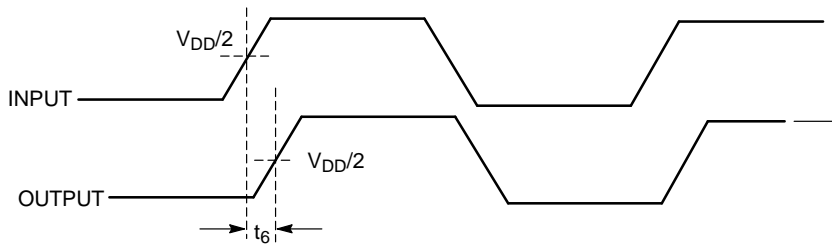
Figure 7. Input-Output Propagation Delay
